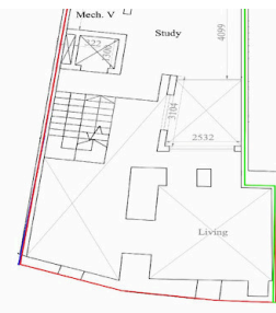
Intermediate Floor Plan As Proposed Scale 1:100
