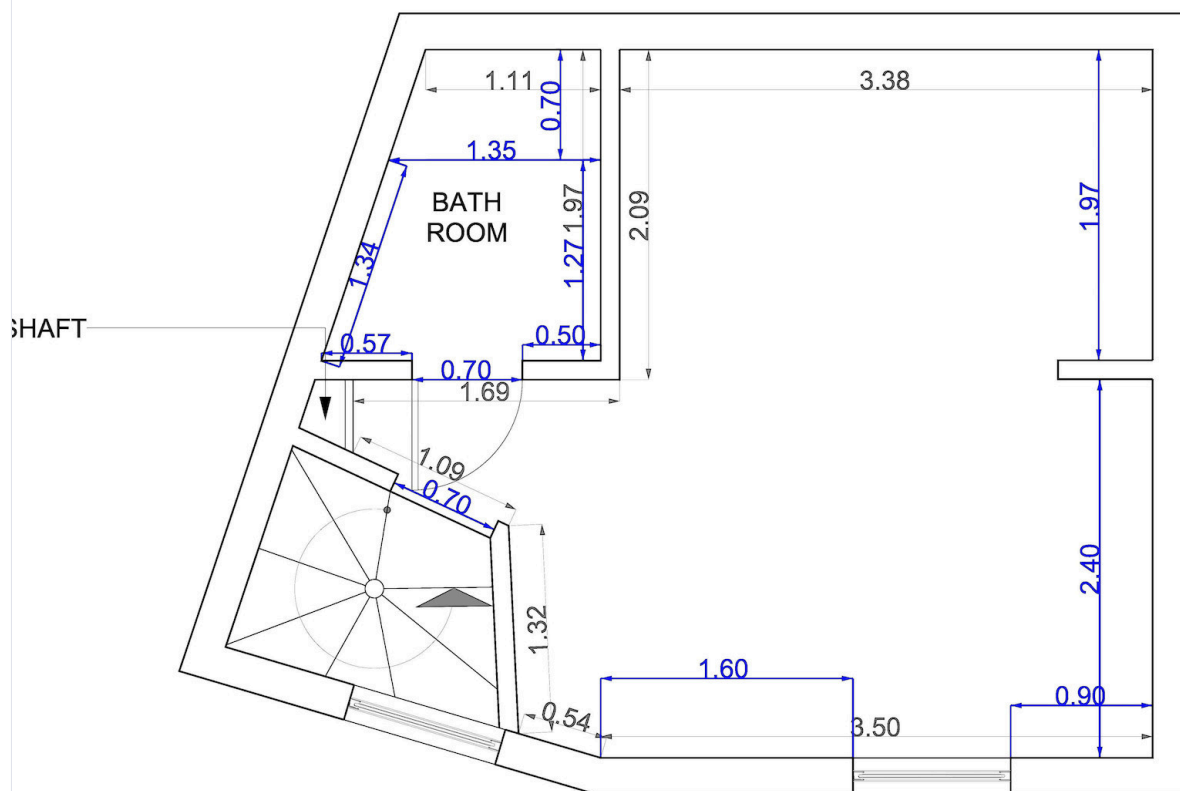
PROPOSED FIRST FLOOR LEVEL
